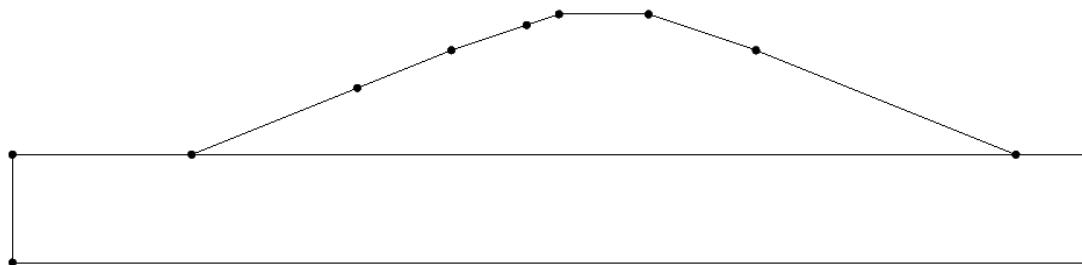
Figure 2. Arcs connecting points.
