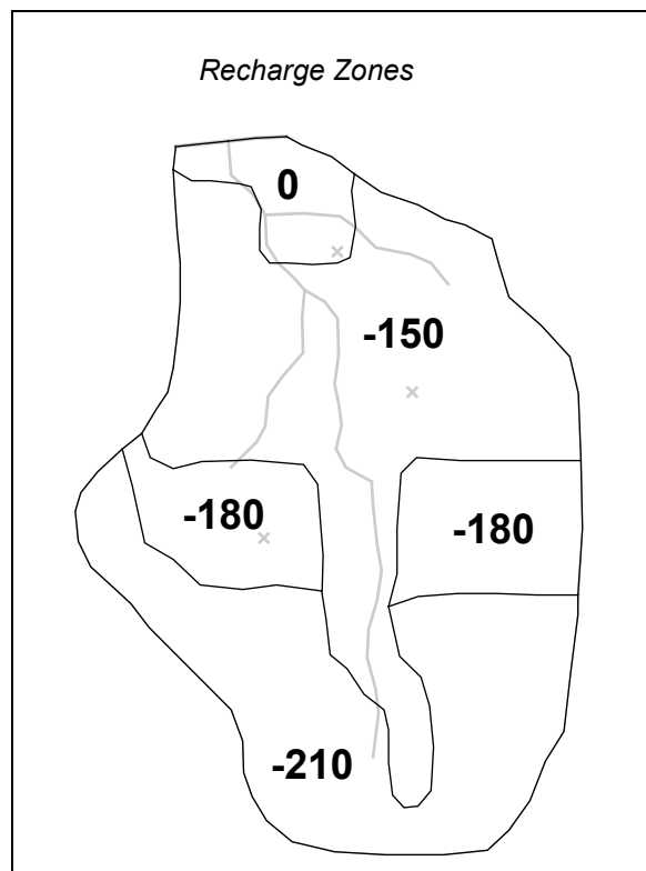
Figure 2. Recharge zones and parameter key values.
